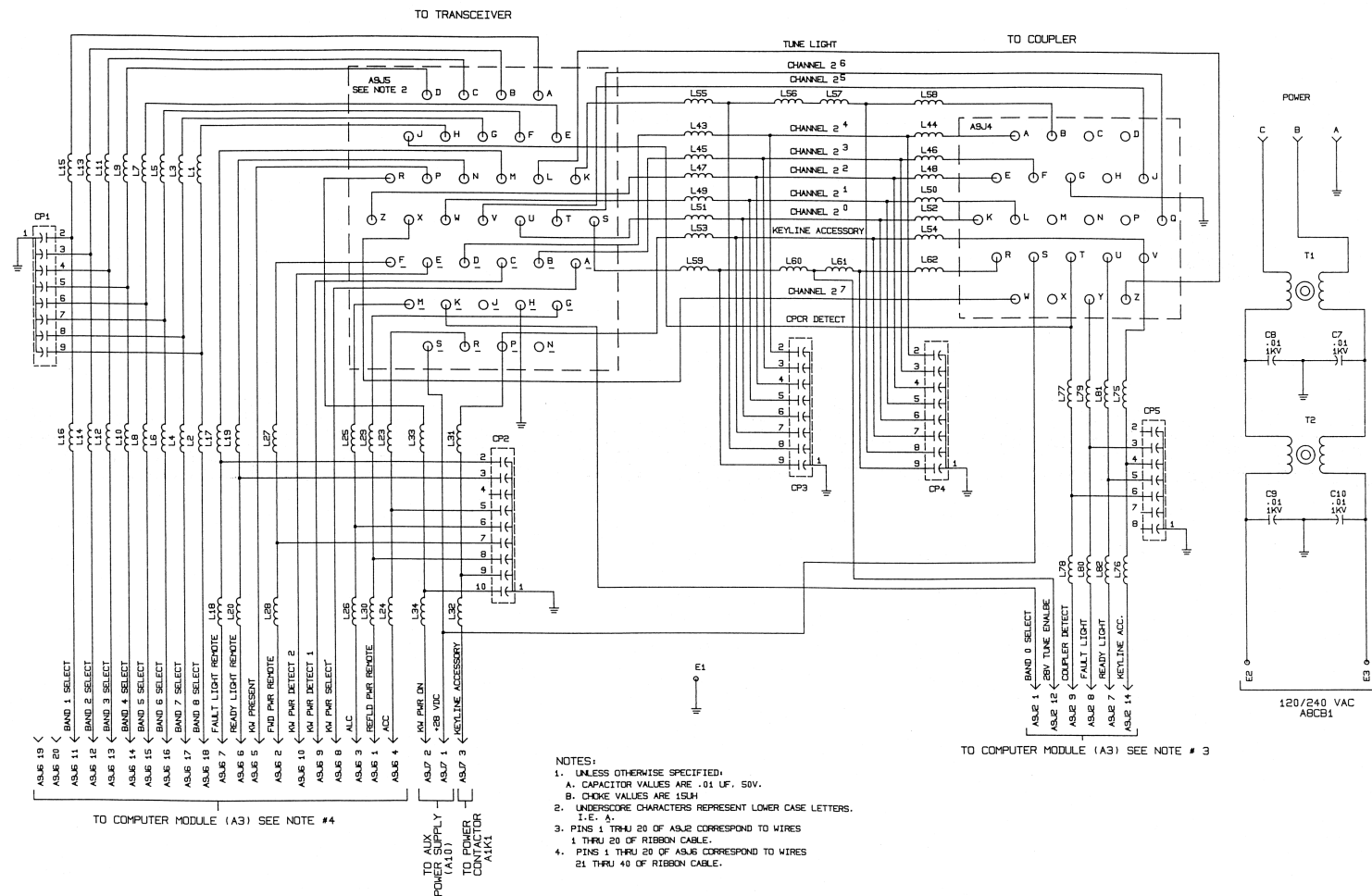
Figure 5.8-23: PC Assembly, Rear Panel Connector, A9
