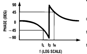
FIGURE 4. 2nd-Order Notch Response
