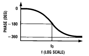
FIGURE 5. 2nd-Order All-Pass Response
