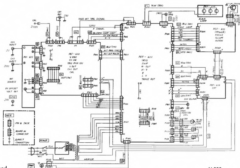
V-222 WIRING DIAGRAM
