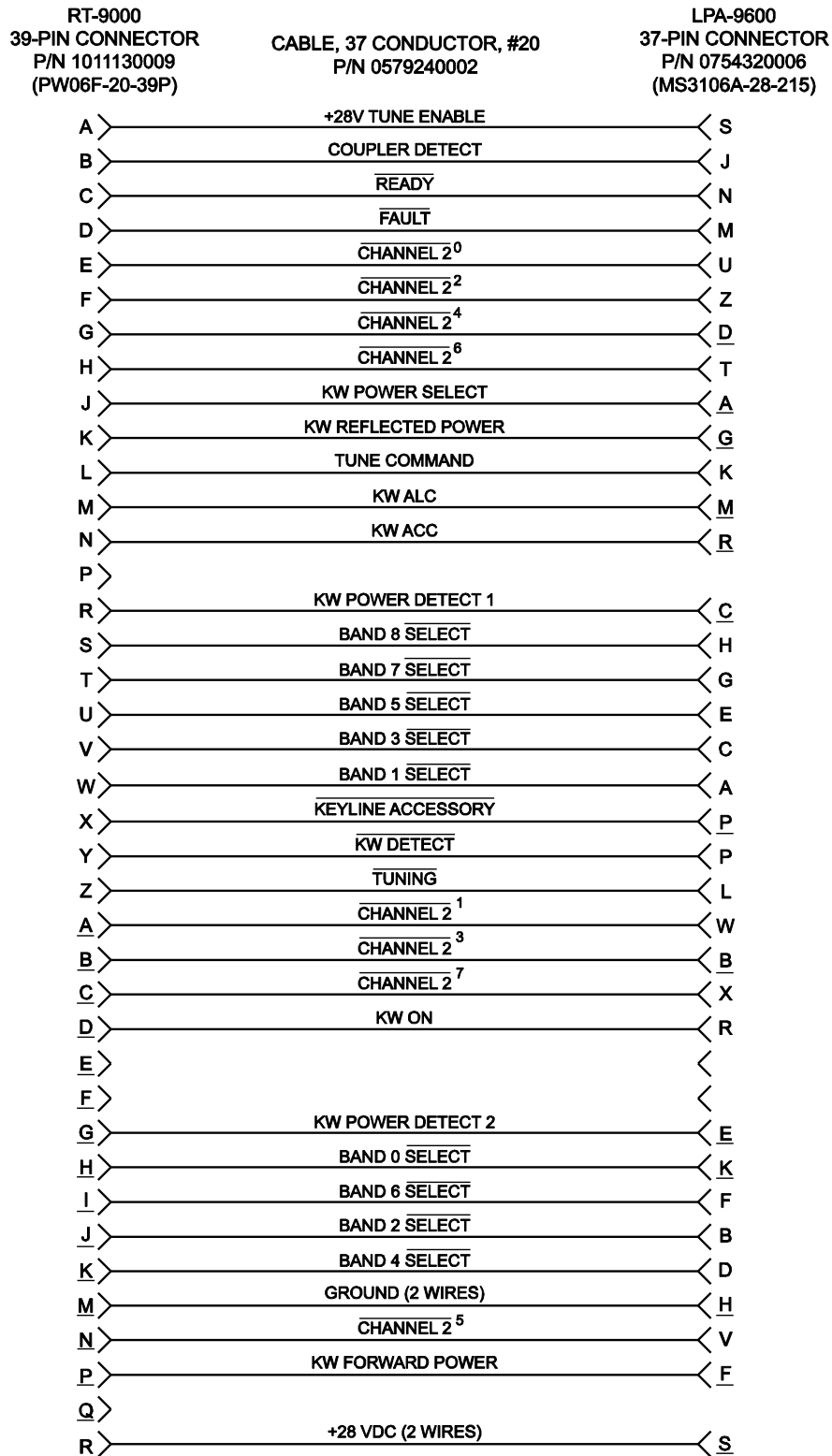
Figure 2.7-2: 9000 Series Exciter/Transceiver to LPA-9600 Control Cable
