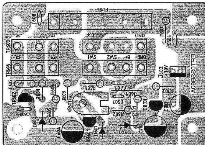
EPTOSSB60A POWER SUPPLY
