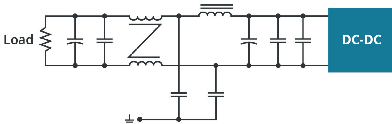
Figure 3 VFM-15C & VFM-25C
